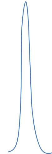
“bursts” with maximal velocities increasing beyond any limit
