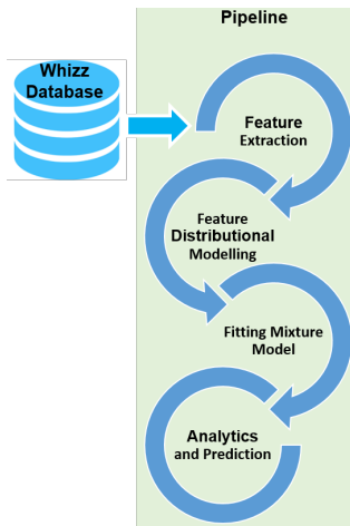
Figure 4 – Modelling Pipeline.
